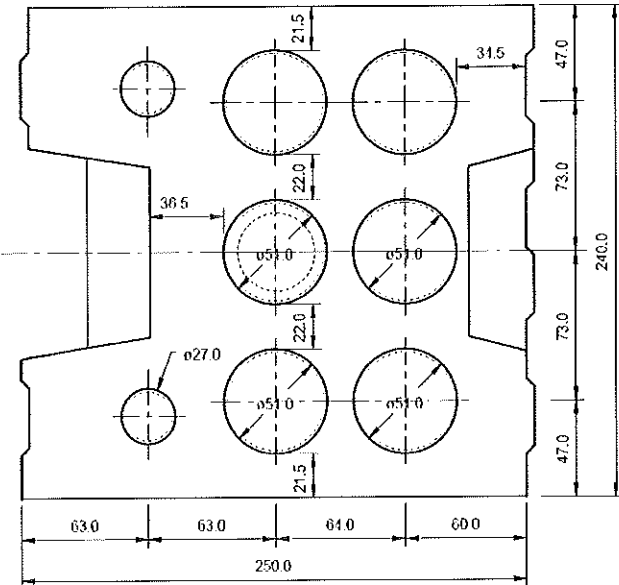
Figure 2 (KSL)
