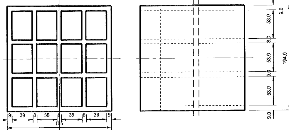
Figure 3 (Brique Creuse)
