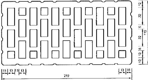
Figure 1 (HLz)
