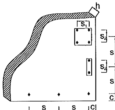
Scheme of distances and spacing in concrete
